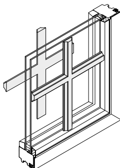
Permanent Exterior Removable Interior
