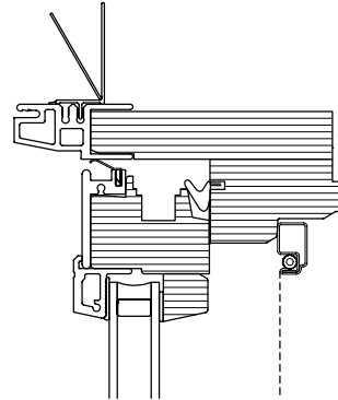
Curved Head Cross Section
