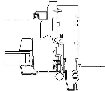
Side Jamb Cross Section
