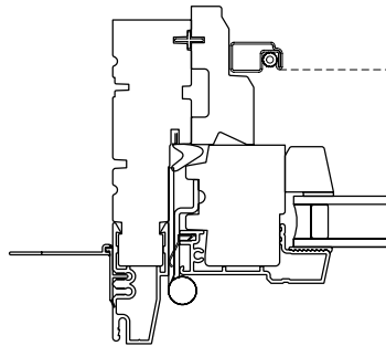
Side Jamb Cross Section
