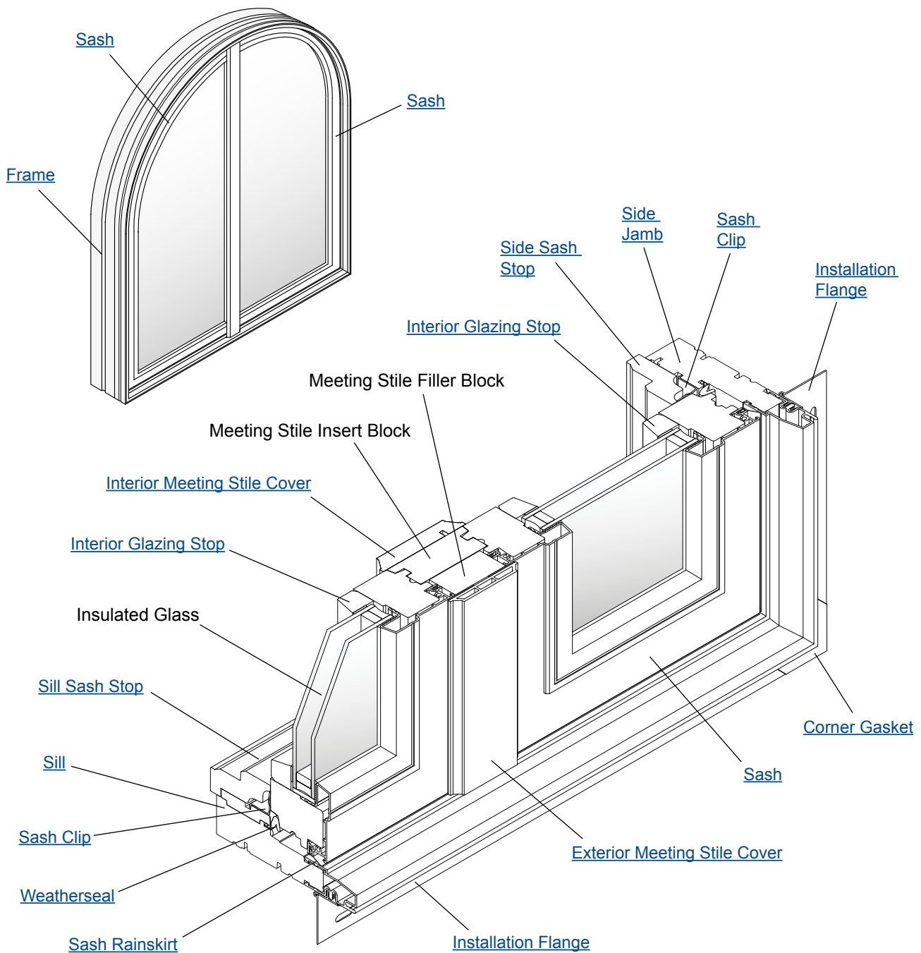
Complementary Clad French Casement Windows Unit Parts - Fixed Windows
