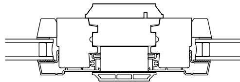
Meeting Stile Cross Section
