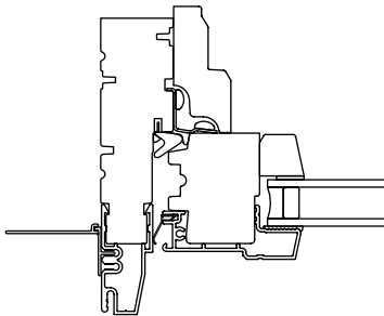
Side Jamb Cross Section
