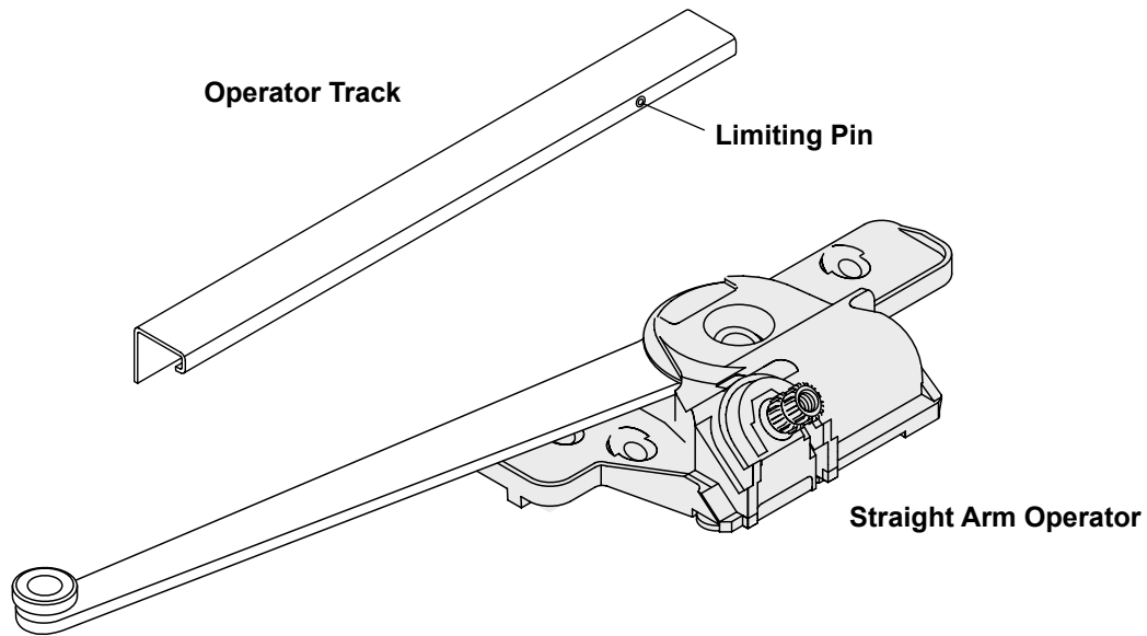
Complementary Clad French Casement Windows - Straight Arm Operator and Track
