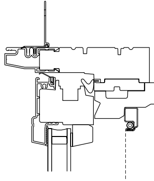
Lineal Head Cross Section
