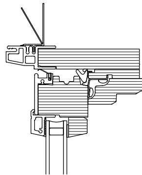
Curved Head Cross Section
