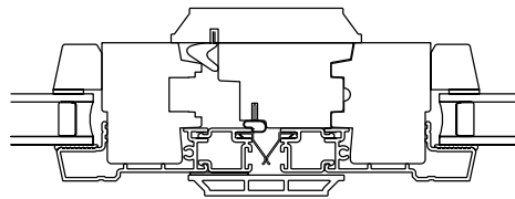
Meeting Stile Cross Section
