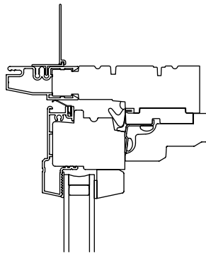
Lineal Head Cross Section
