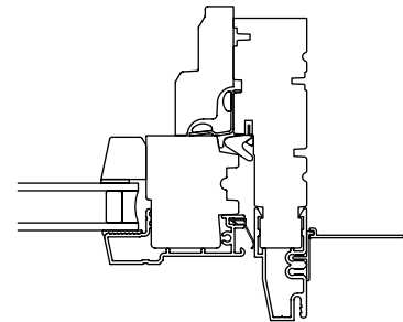
Side Jamb Cross Section
