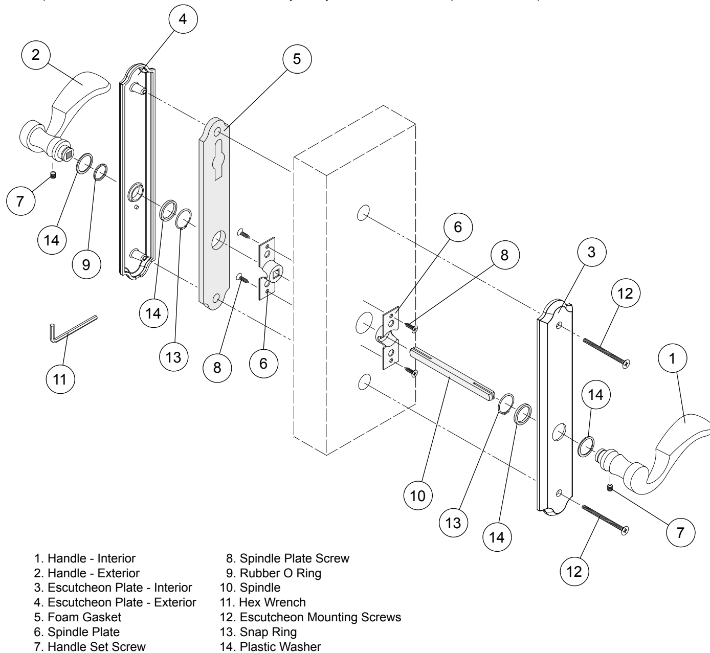
Clad Outswing Entry Doors - Dummy Trim Set
