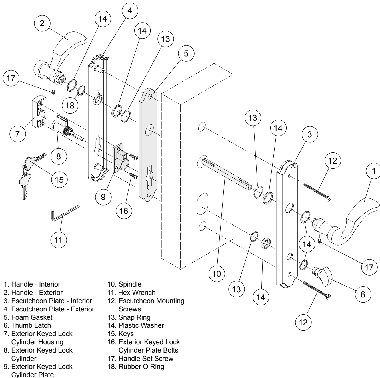
Clad Outswing Entry Doors - European Active Trim Set
