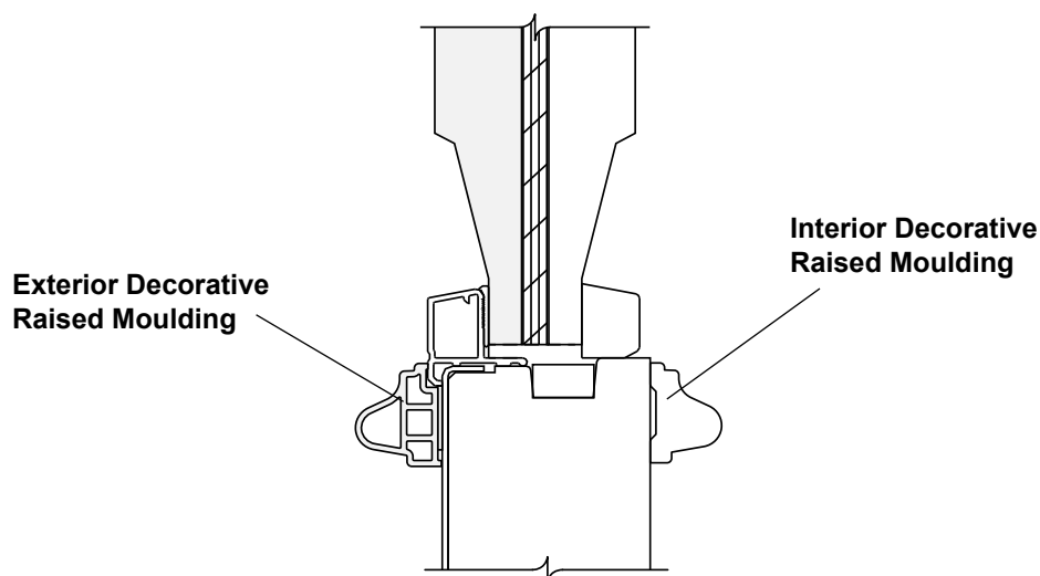
Clad Outswing Entry Doors - Decorative Raised Mouldings
