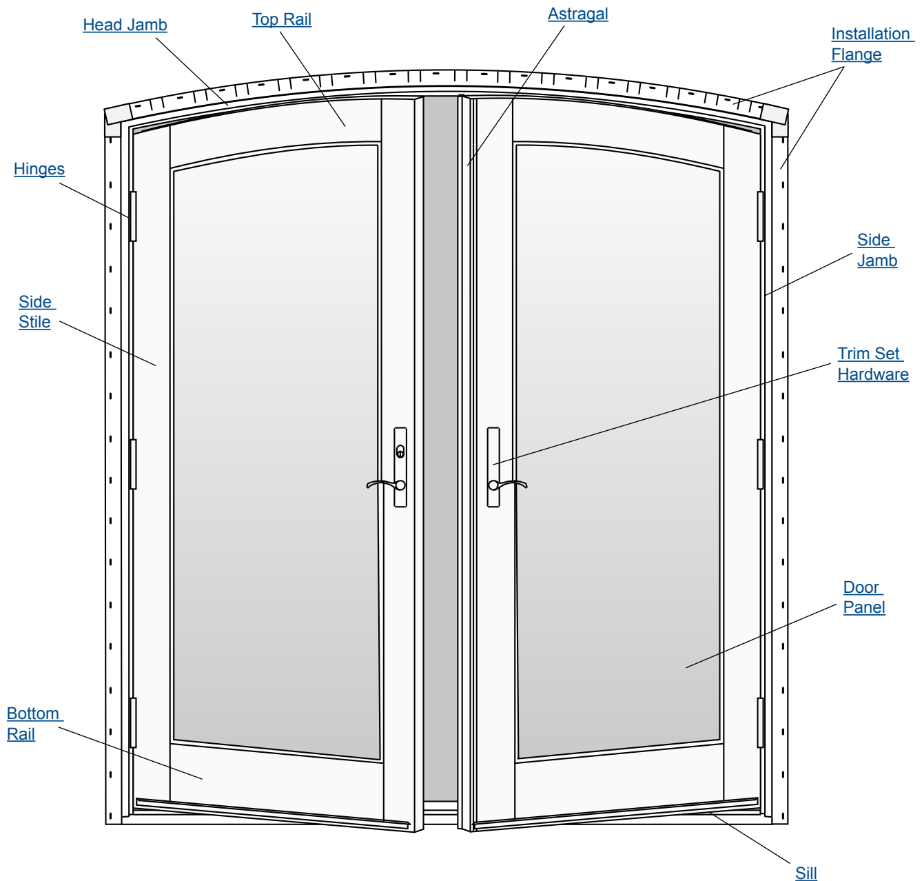
Manufactured 2001 to Present Clad Outswing Entry Doors Unit Parts - Double Doors
