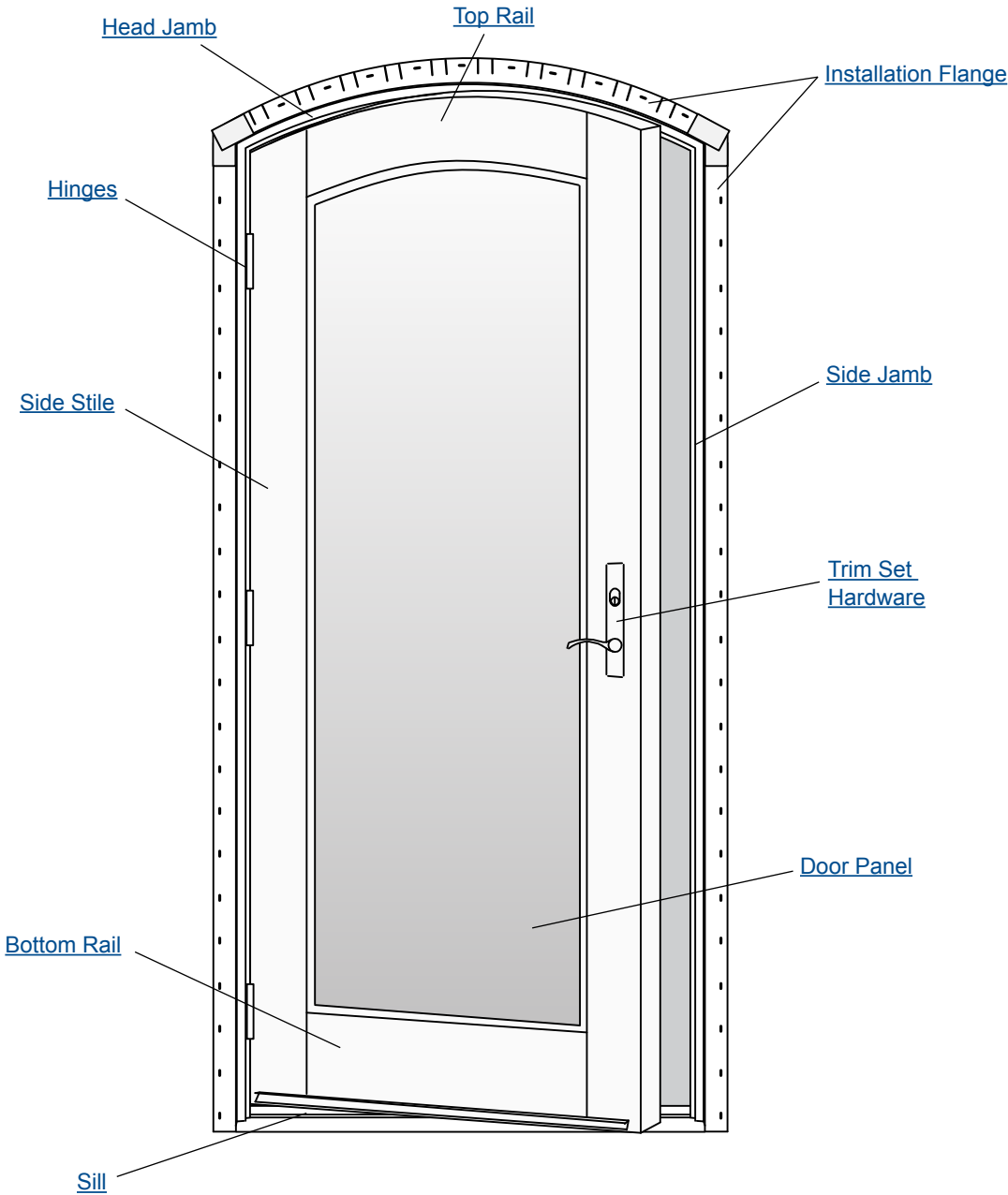
Manufactured 2001 to Present Clad Outswing Entry Doors Unit Parts - Single Door
