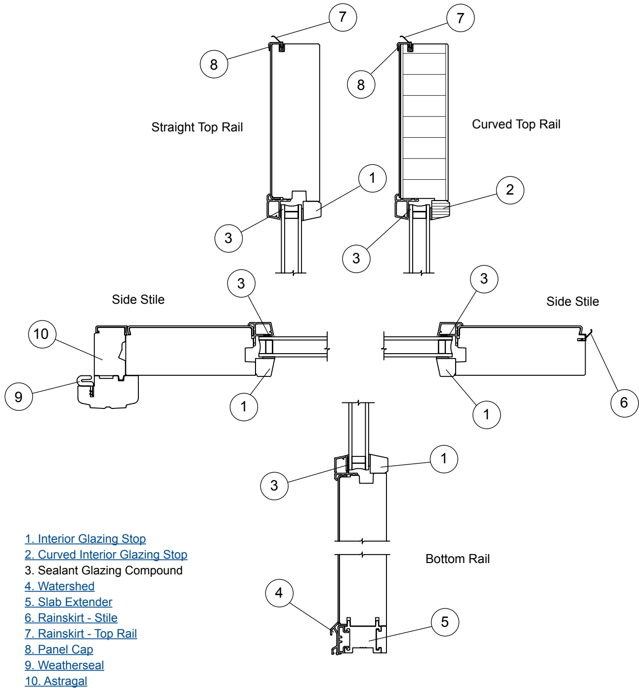
Clad Outswing Entry Doors - Passive Panels
