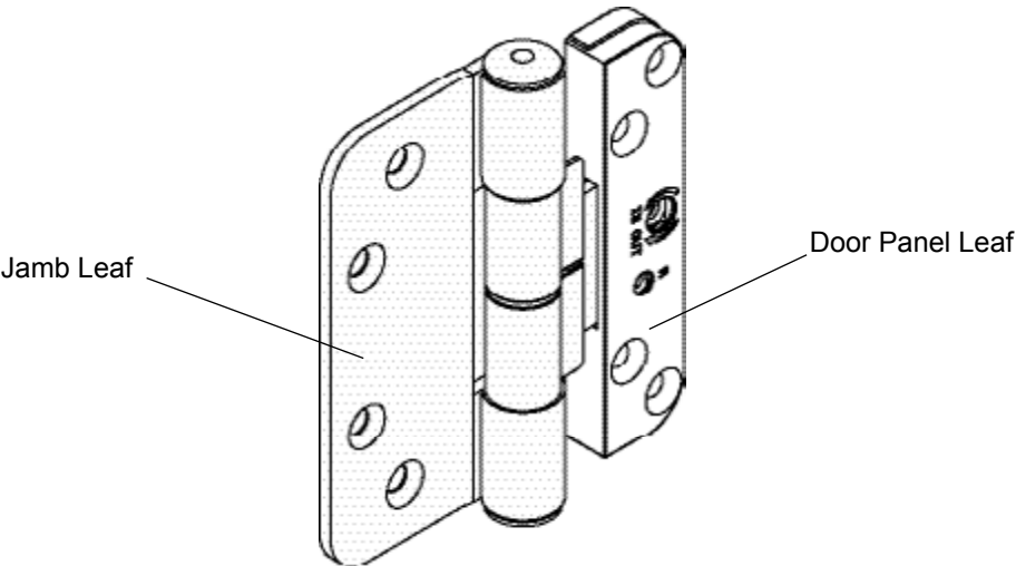
Wood Inswing Entry Doors - Adjustable Hinge
