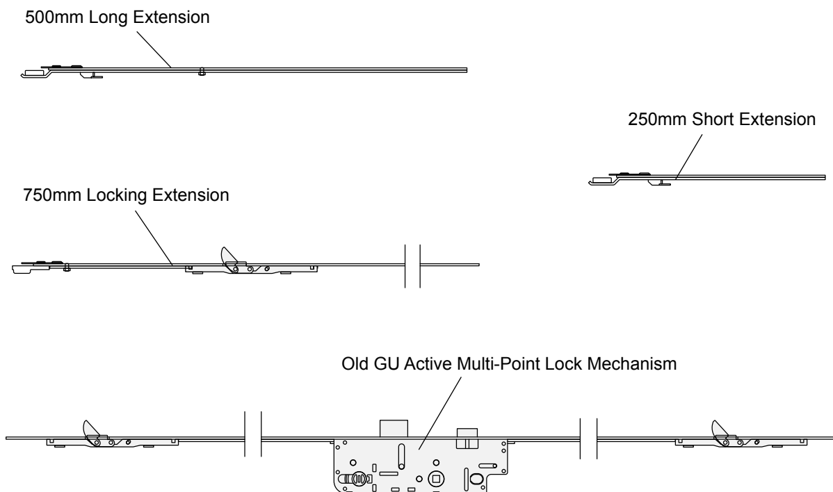
Wood Inswing Doors - Old GU Active Lock Assembly
