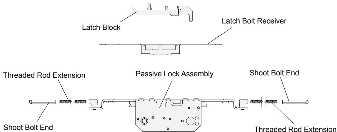
Wood Inswing Doors - AW Passive Lock Assembly
