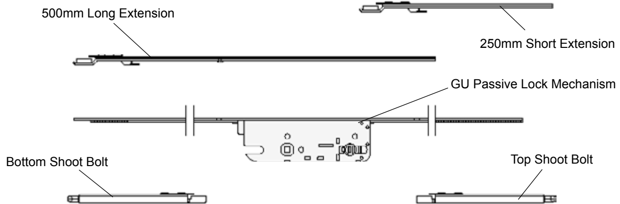
Wood Inswing Entry Doors - GU Passive Lock Assembly
