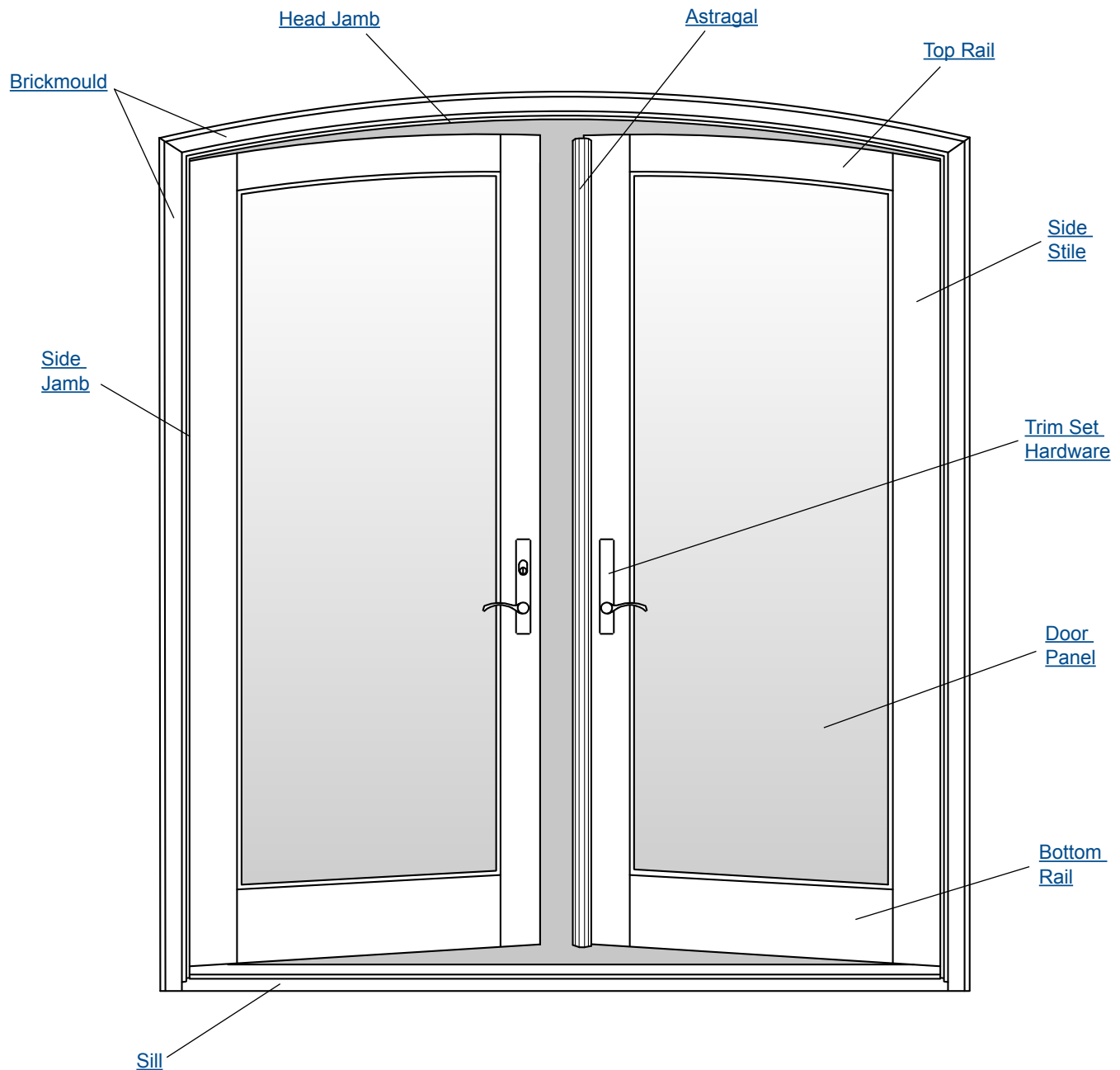
Manufactured 2001 to Present Wood Inswing Doors Unit Parts - Double Doors
