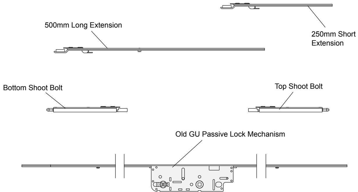
Wood Inswing Doors - Old GU Passive Lock Assembly
