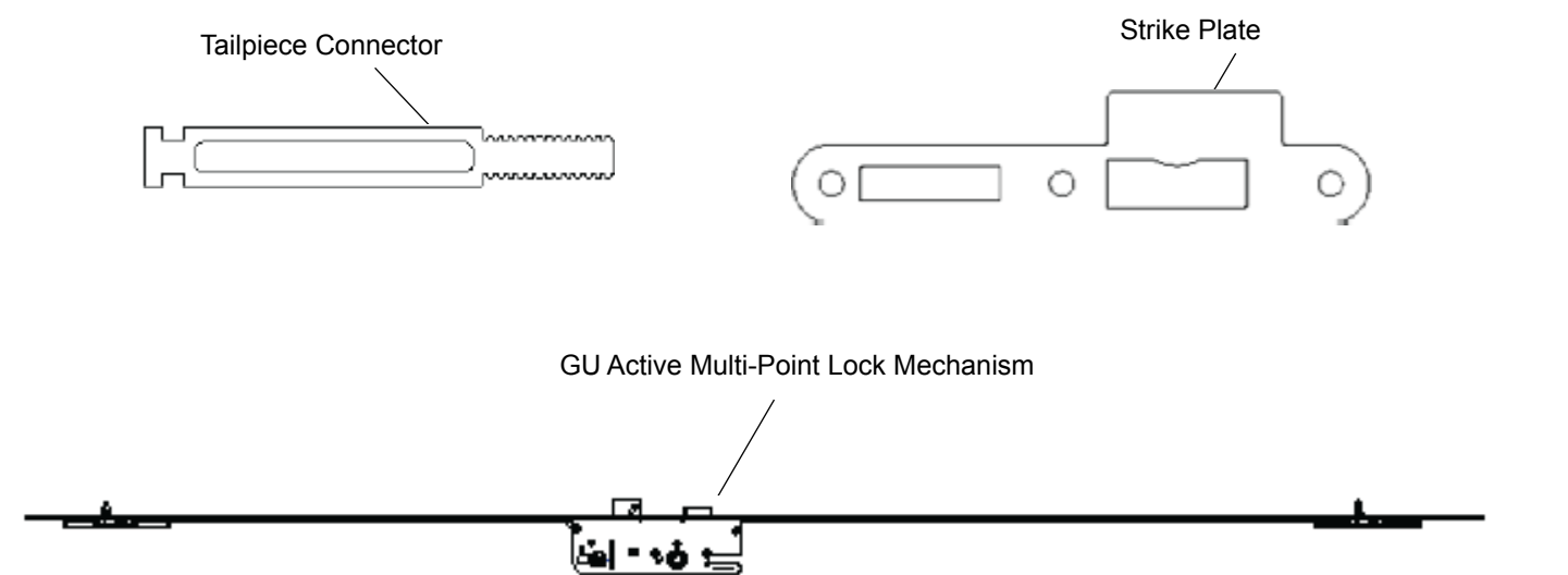
Wood Inswing Entry Doors - Old GU Active Lock Assembly
