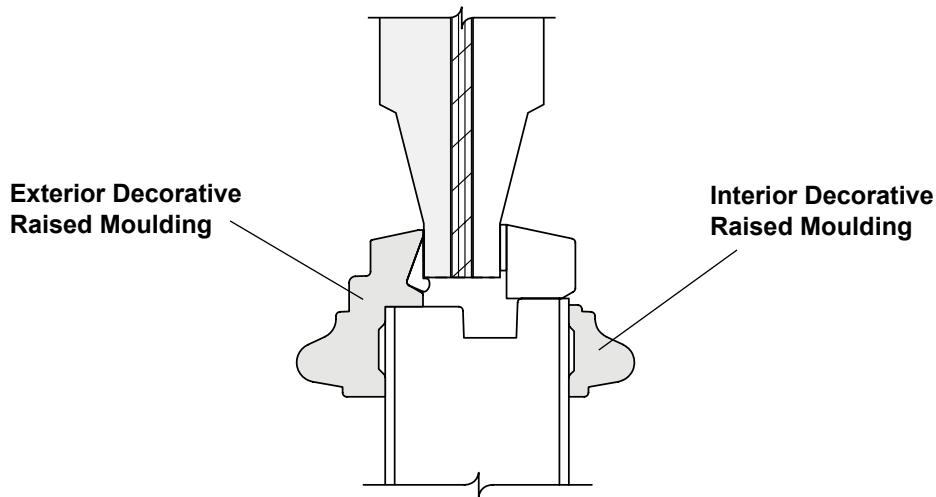
Wood Inswing Doors - Decorative Raised Mouldings
