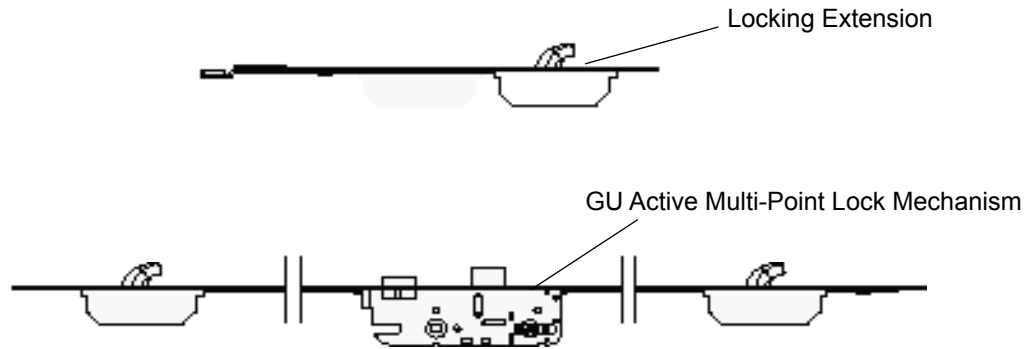
Wood Inswing Entry Doors - GU Active Lock Assembly
