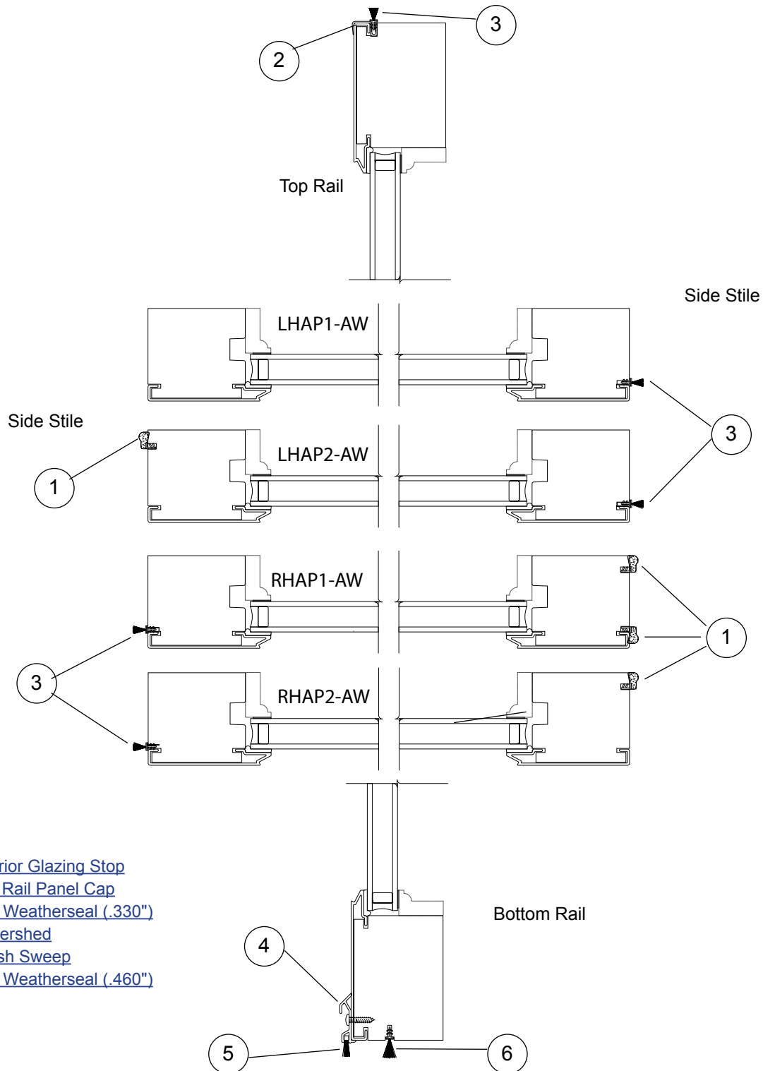
Clad Outswing Folding Doors - Active Panels
