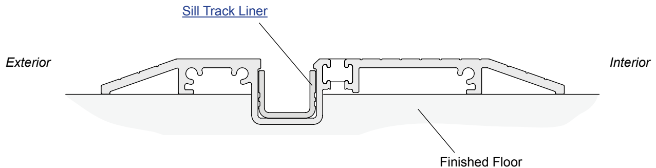
Clad Outswing Folding Doors - Low Profile Sill
