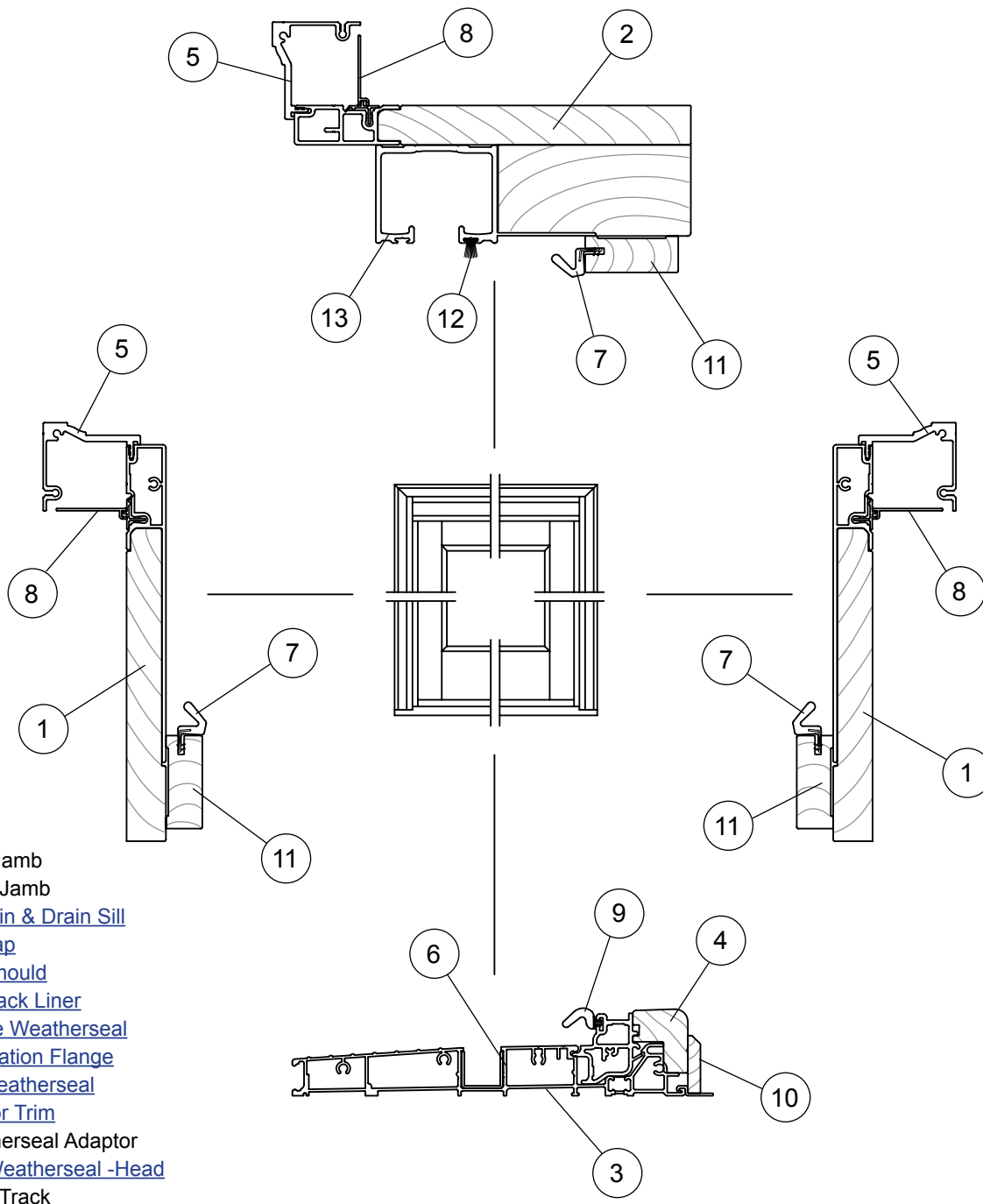
Clad Outswing Folding Doors - 6 9 / 16 " Wall Thickness / 2 1 / 4 " Door Panels
